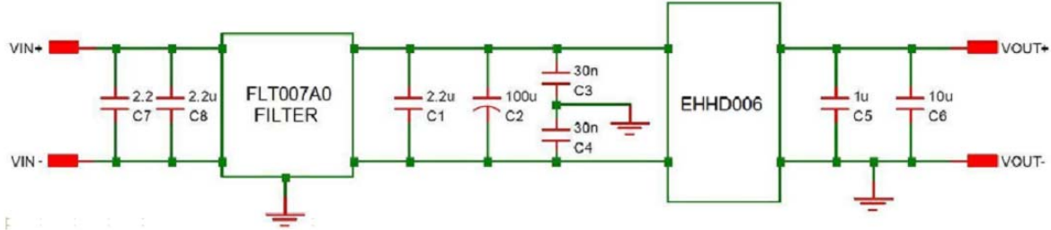
Figure 26. EMC Considerations
